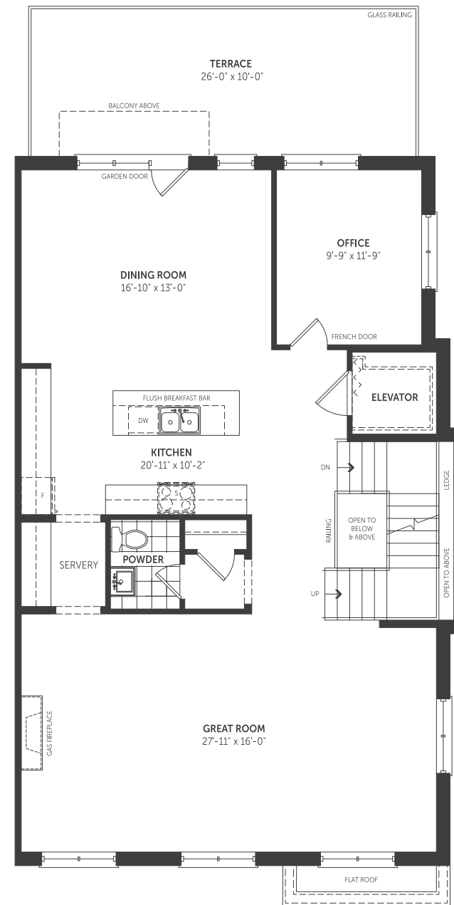
SECOND FLOOR 1,398 SQFT
