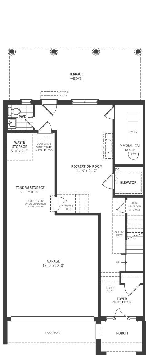
OPT. GROUND FLOOR 665 SQFT
