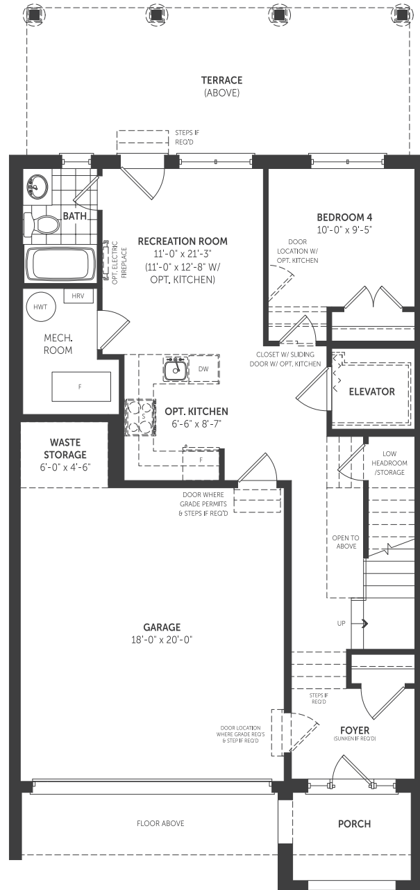
GROUND FLOOR 800 SQFT
