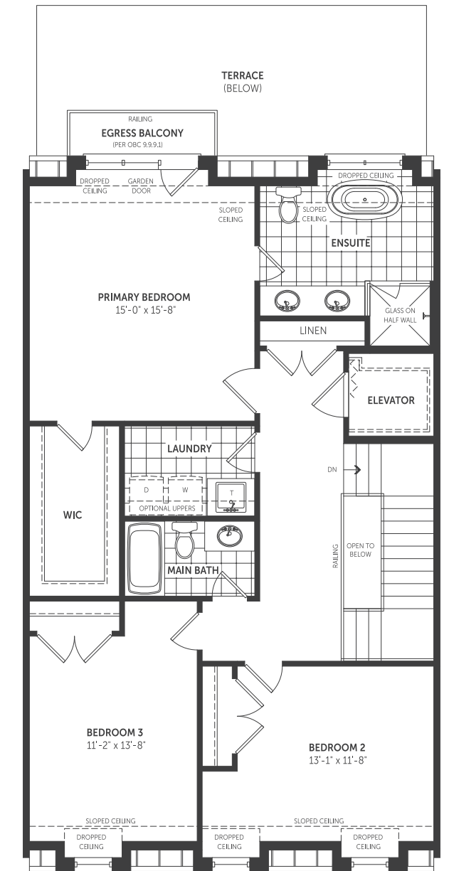
THIRD FLOOR 1,290 SQFT
