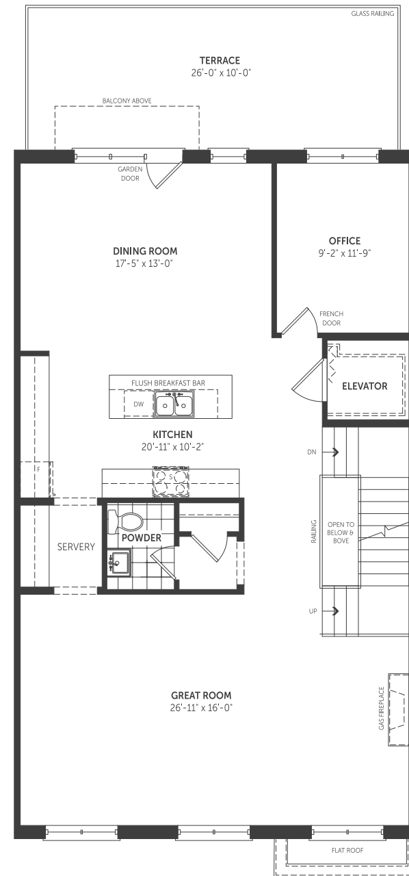
SECOND FLOOR 1,323 SQFT
